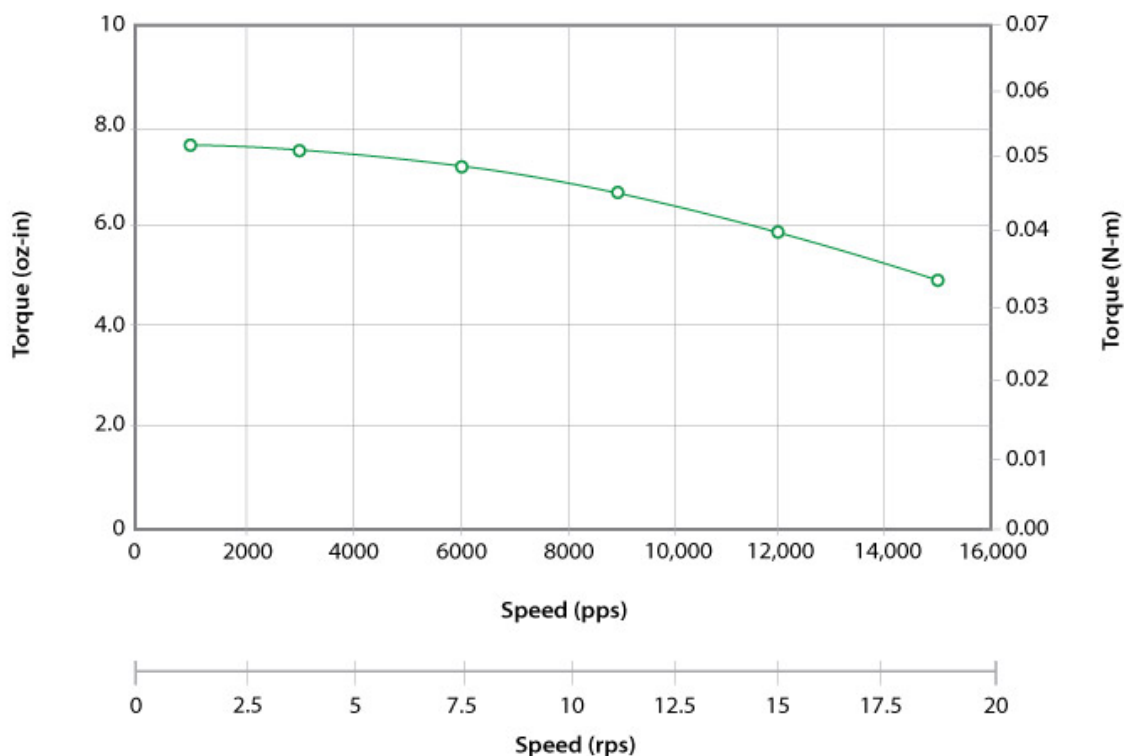
3809X-51 24VDC, 0.6 Amps/Phase, Bipolar, 1/2 Stepping
